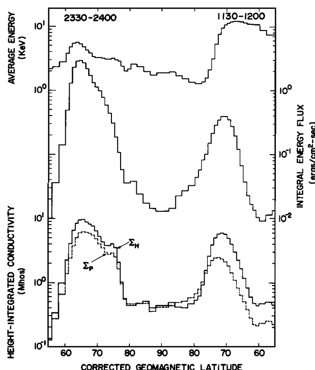
Fig. 3. The Hall and Pedersen conductivities along the noon-midnight meridian plotted along with the energy flux and average energy for precipitating electrons with energies greater than 661 eV for Kp = 3 .
